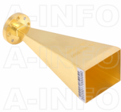
LB-10-25-A Standard Gain Horn Antenna 75-110GHz 25dB Gain Rectangular Waveguide Interface
